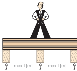
2-Feld-System
